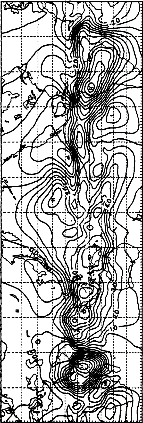
VELOCITY POTENTIAL 200MB DEC 1980
